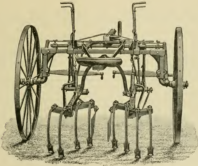
DOUBLE CORN CULTIVATOR.
